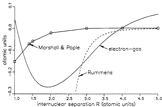
Figure 2. Theoretical calculations of the prototypical intermolecular shielding function, proton shielding in triplet H_2 molecule as a function of internuclear distance (reprinted from ref 35; copyright 1991 Academic Press). The electron gas calculation provides a shielding function that has the same form as the one derived from direct inversion of experimental data for the rare gas pair Xe-Xe.
