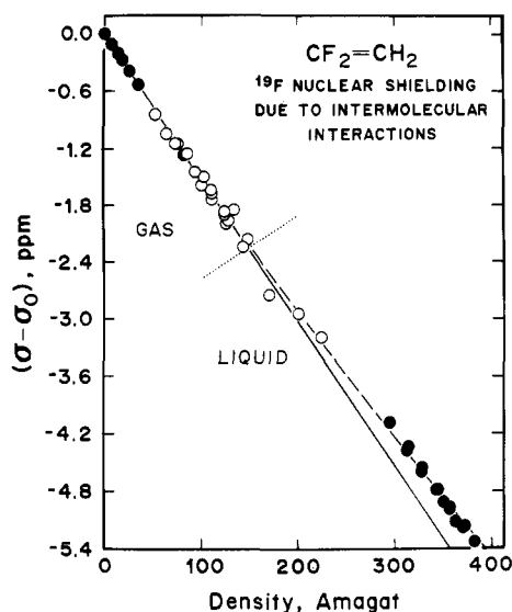
Figure 1. The density dependence of the ^{19}\text{F} nuclear shielding in \text{CF}_2=\text{CH}_2 . The critical point is 303.3 K and 146 amagat. Open circles and filled circles correspond to independent measurements from two laboratories (reprinted from ref 8; copyright 1984 American Institute of Physics).
