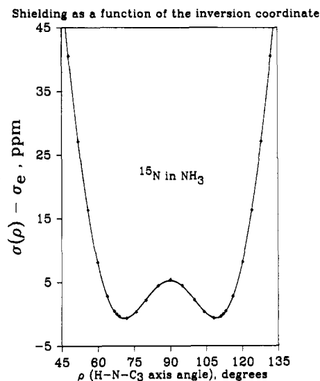
Figure 7. A trace on the ab initio nitrogen shielding surface along the inversion coordinate of ammonia molecule, calculated by using the LORG method (reprinted from ref 43; copyright 1991 American Institute of Physics).
